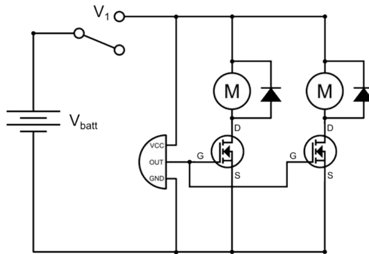
Figure 10. A complete circuit diagram for the motion-activated robot.
