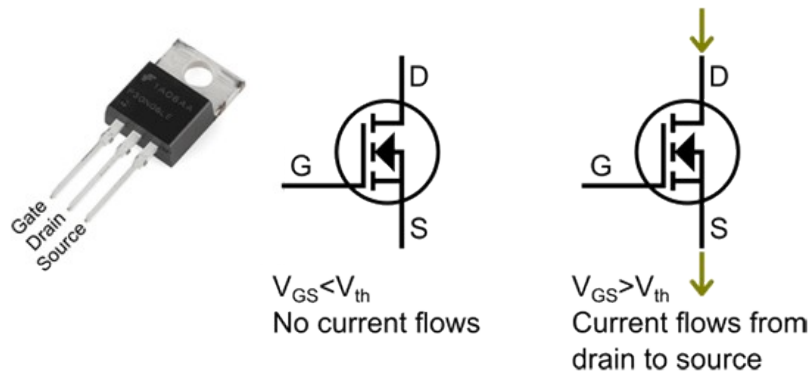
Figure 9. Simplified explanation of a MOSFET's operation.
