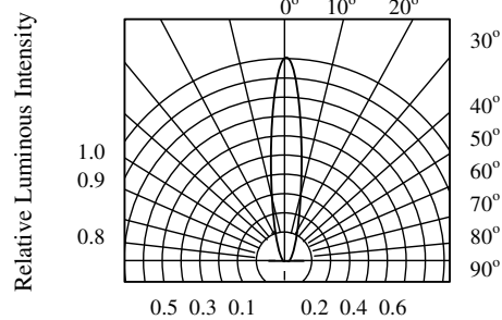
FIG.6 RADIATION DIAGRAM
